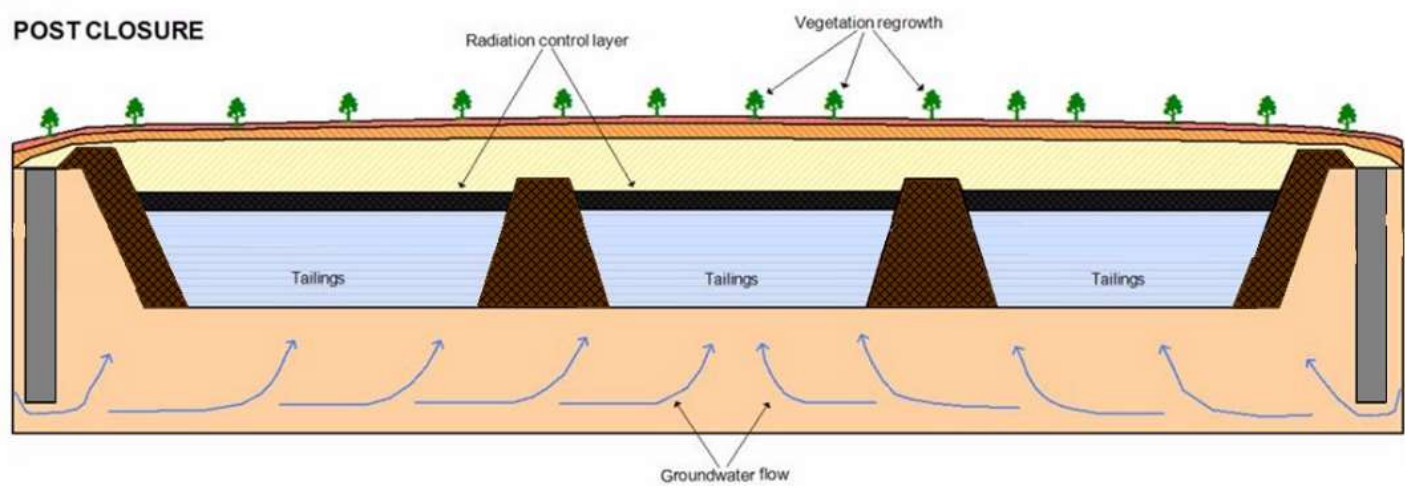
Figure 1: Tailings Storage Diagram
