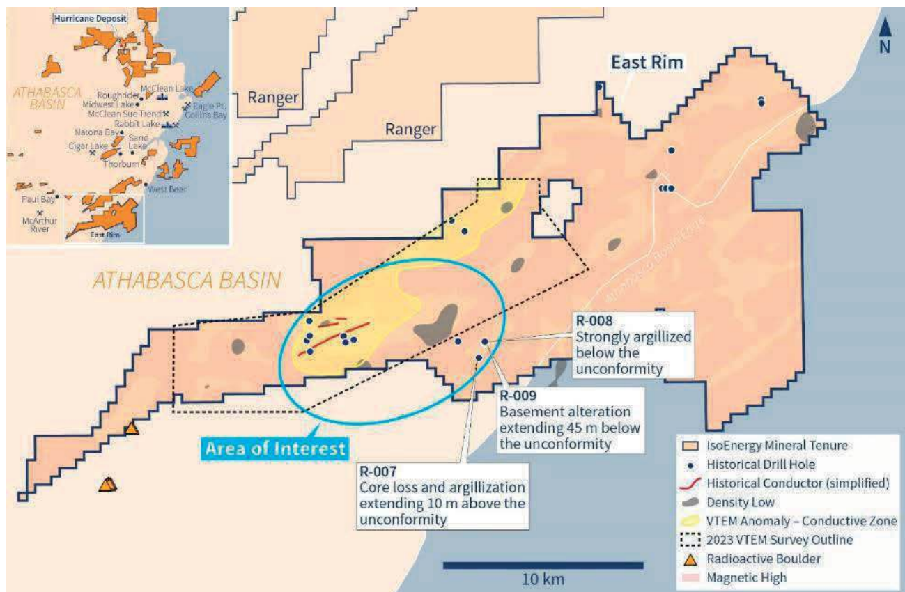
Figure 14: East Rim project, area of interest Source: IsoEnergy website
