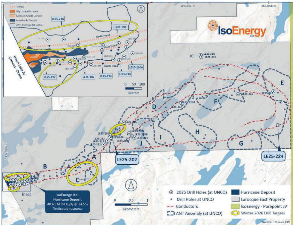
Figure 11: Compilation map of Larocque East project, 2024 / 2025 drilling and ANT anomalies
