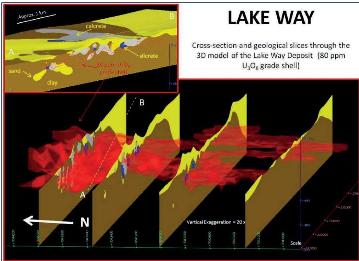
Figure 5: Resource Model Lake Way Deposit showing U_3O_8 Grade
