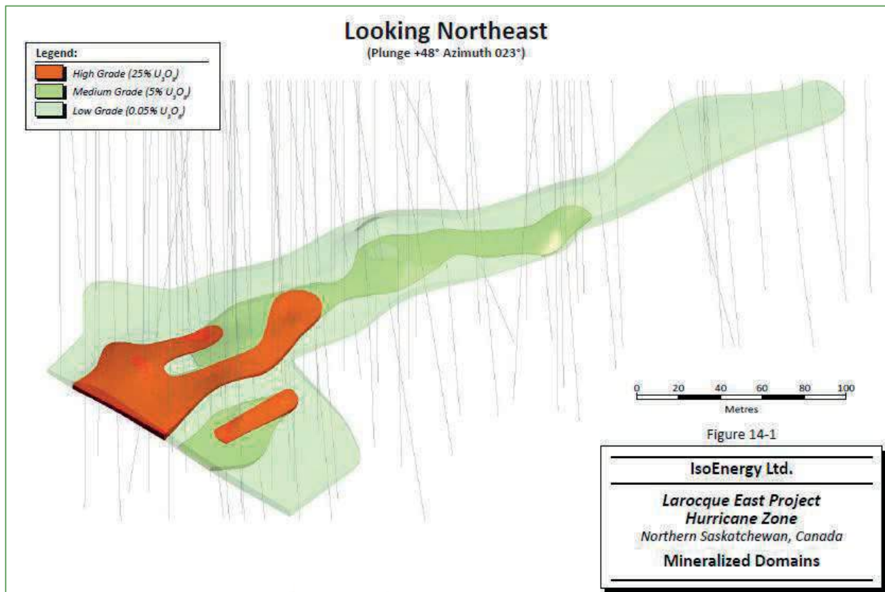
Figure 12: Larocque East (Hurricane) interpreted mineralisation envelopes
