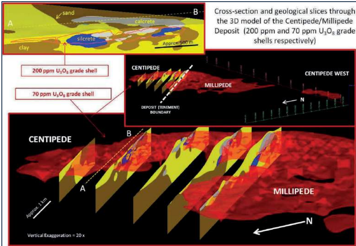
Figure 4: Resource Model - Centipede-Millipede Deposit showing U_3O_8 Grade
