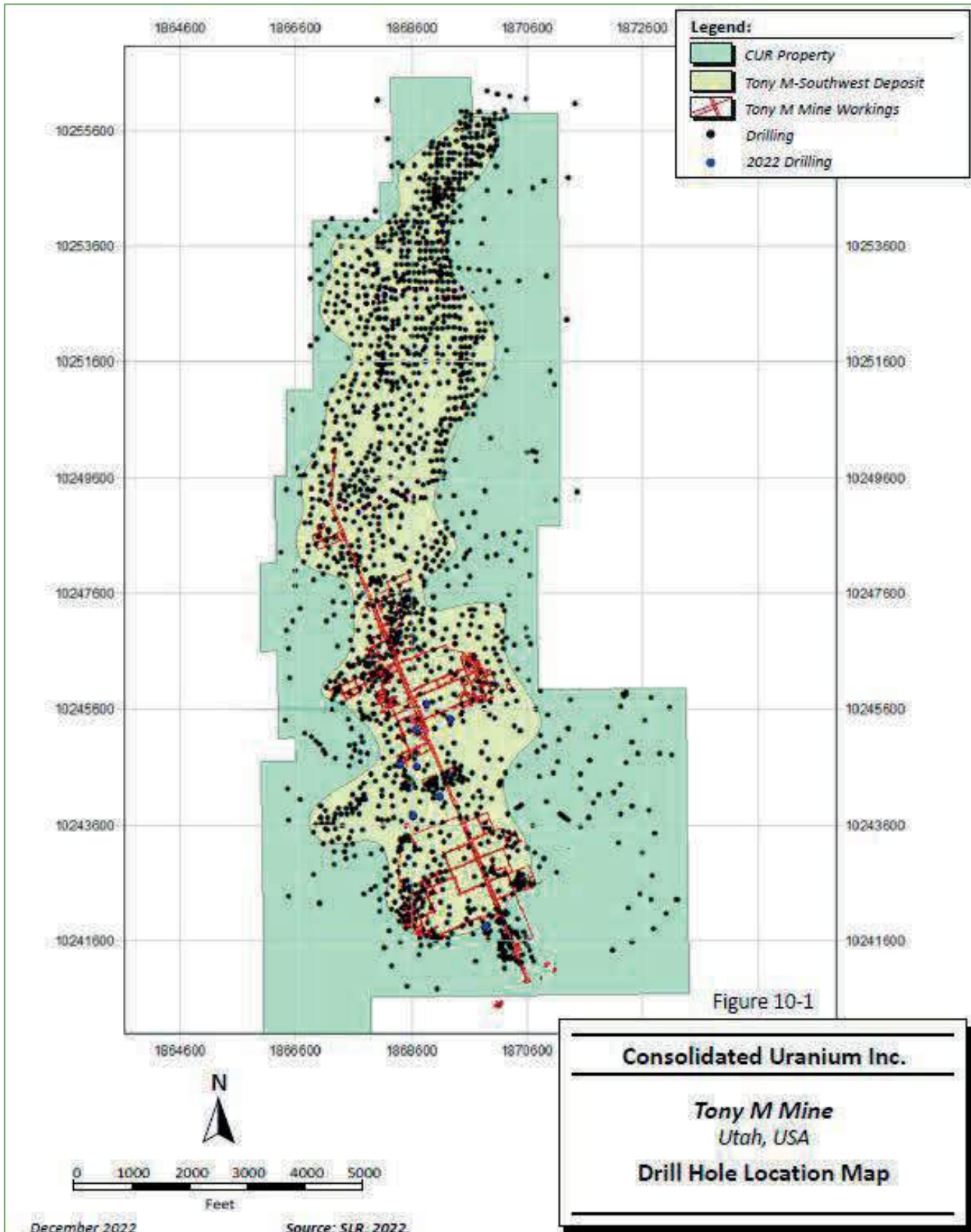
Figure 26: Tony M drillhole collar locations Source: SLR, 2022
