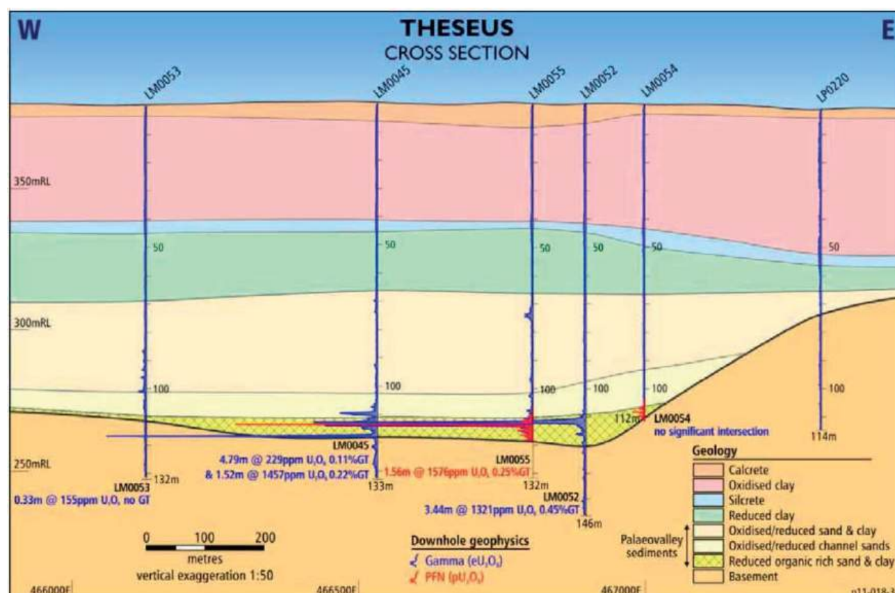
Figure 6 : Theseus Deposit Geological Cross Section showing Drilling Results
